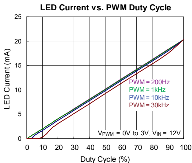
Figure 2. LED Current vs. PWM Dimming Duty Cycle
