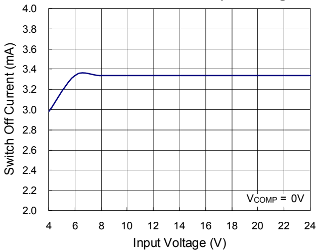
Switch Off Current vs. Input Voltage
