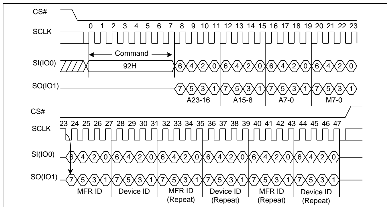
Figure 28. Read Manufacture ID/ Device ID Dual I/O Sequence Diagram
