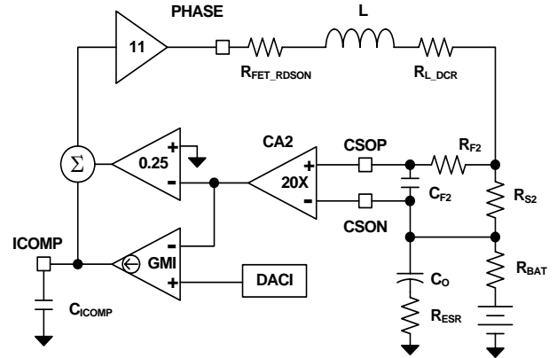
FIGURE 21. CHARGE CURRENT LIMIT LOOP
