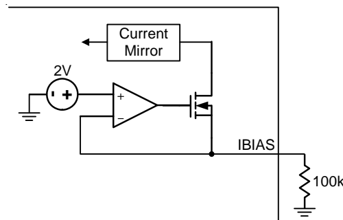
Figure 2. IBIAS Setting
